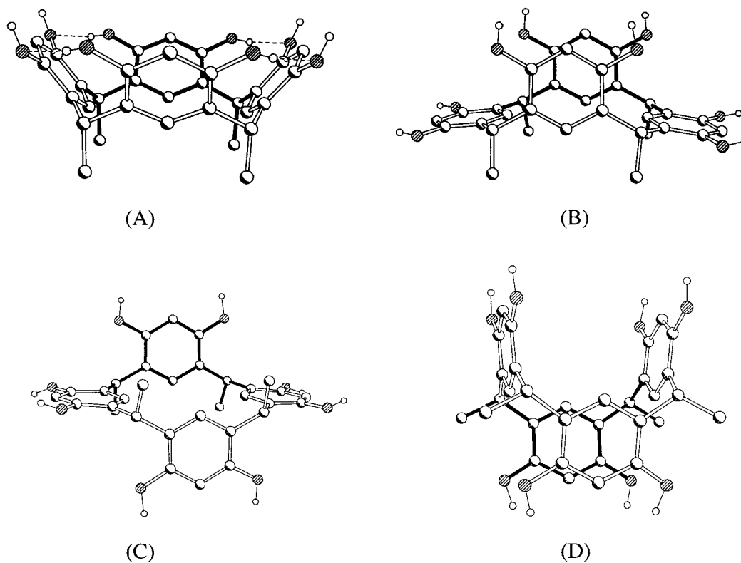
Figure 4. Schematic drawing of the four conformations of C -methylcalix[4]resorcinarene: (A) crown; (B) boat; (C) chair; (D) saddle.
