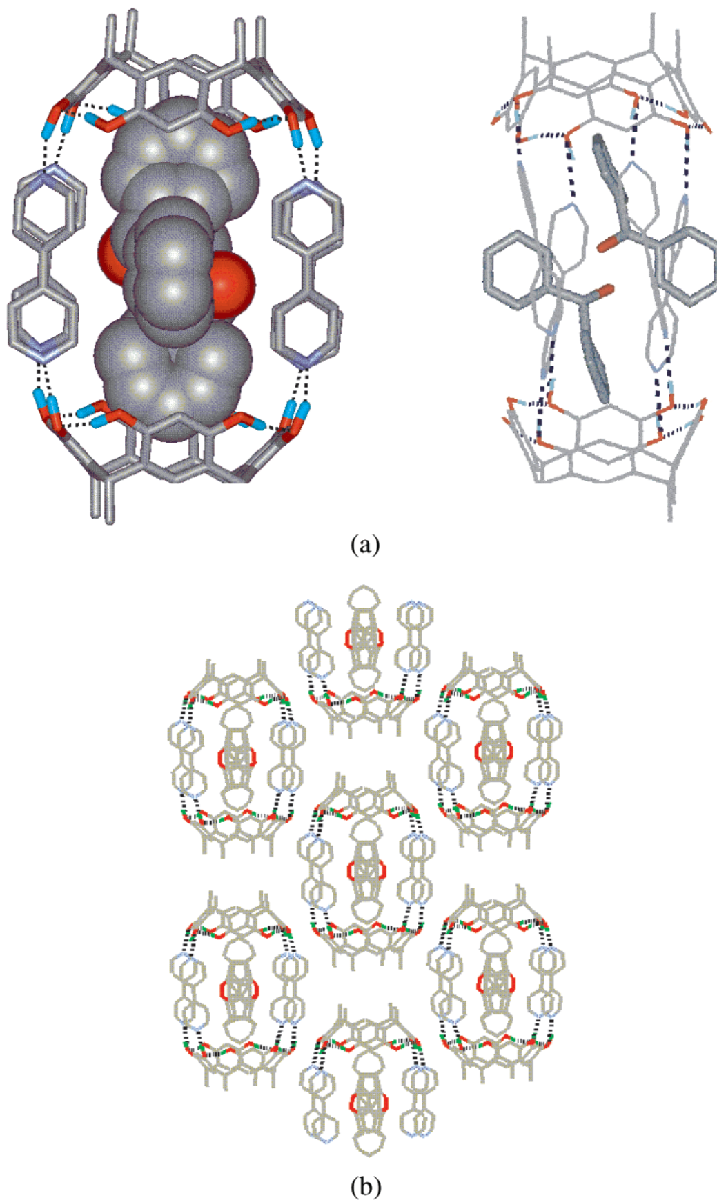
Figure 3. (a) Two different views of the carcerand-like capsule in 3 , formed by hydrogen bonding between CMCR and bipyridine. The capsule has the crystallographic point-symmetry 222 . The two benzophenone molecules included in the cavity each occupy two disordered positions related by one of the 2-fold axes. Only one of the positions for each is shown. (b) The face-centered packing of the capsules in the ab plane. Successive sheets are stacked into a three-dimensional face-centered arrangement.
