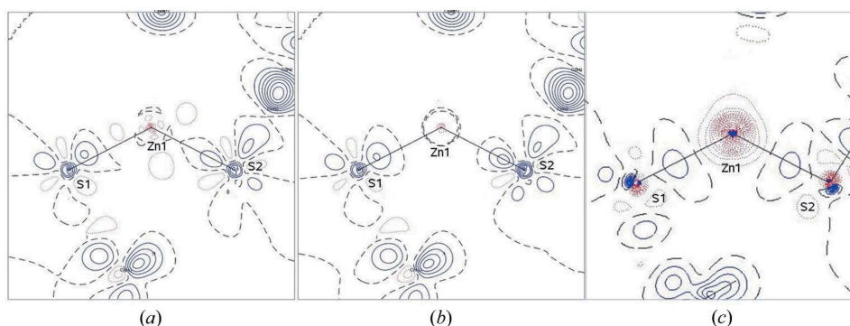
Figure 5 Deformation density maps in the S–Zn–S plane, (a) refinement 3, (b) refinement 2 and (c) theory; contours at 0.1 \text{ e } \text{Å}^{-3} . Blue: excess density, red: deficient density. Zero contours broken.
